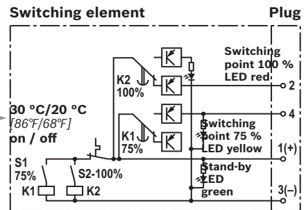
WE-2SPSU-M12x1
