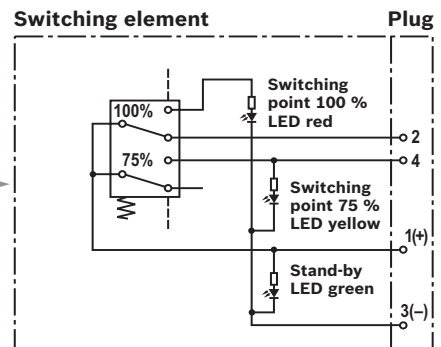
WE-2SP-M12x1
