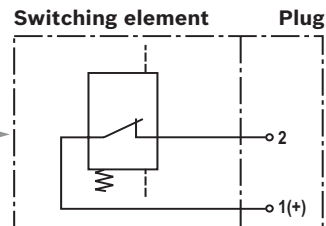
WE-1SP-EN175301-803
