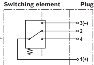
WE-1SP-M12x1
