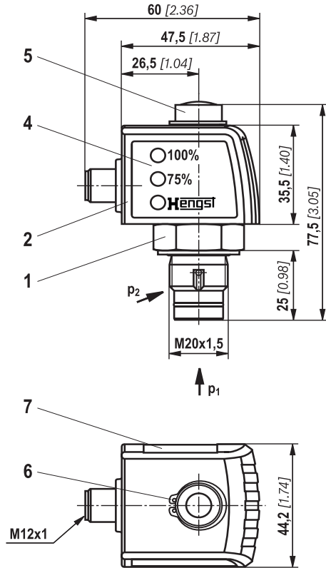
Pressure differential indicator with mounted M12x1 switching element
